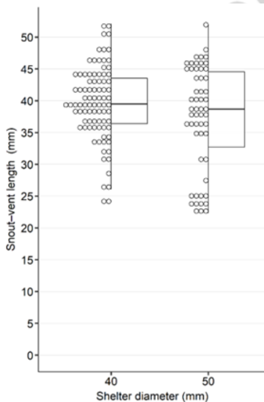
Fig. 3. Snout-vent length (SVL) distribution of H. arborea individuals captured in paired shelter sites (40 mm and 50 mm).
