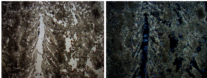
Fig. 34 Sample of 'kanjur' rock, analysis of the microstructure: cone-like structure of calcite sheets with a central channel. Petrographic microscope image: left image: 1 polar; right image + polars (images are 6.8 mm across).
